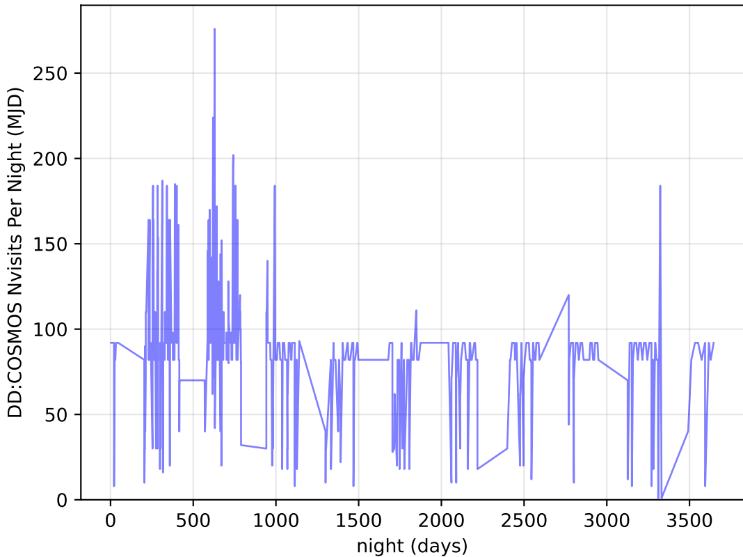
weather_cloudso14v3.4_10yrs all bands: DD: COSMOS Nvisits Per Night
