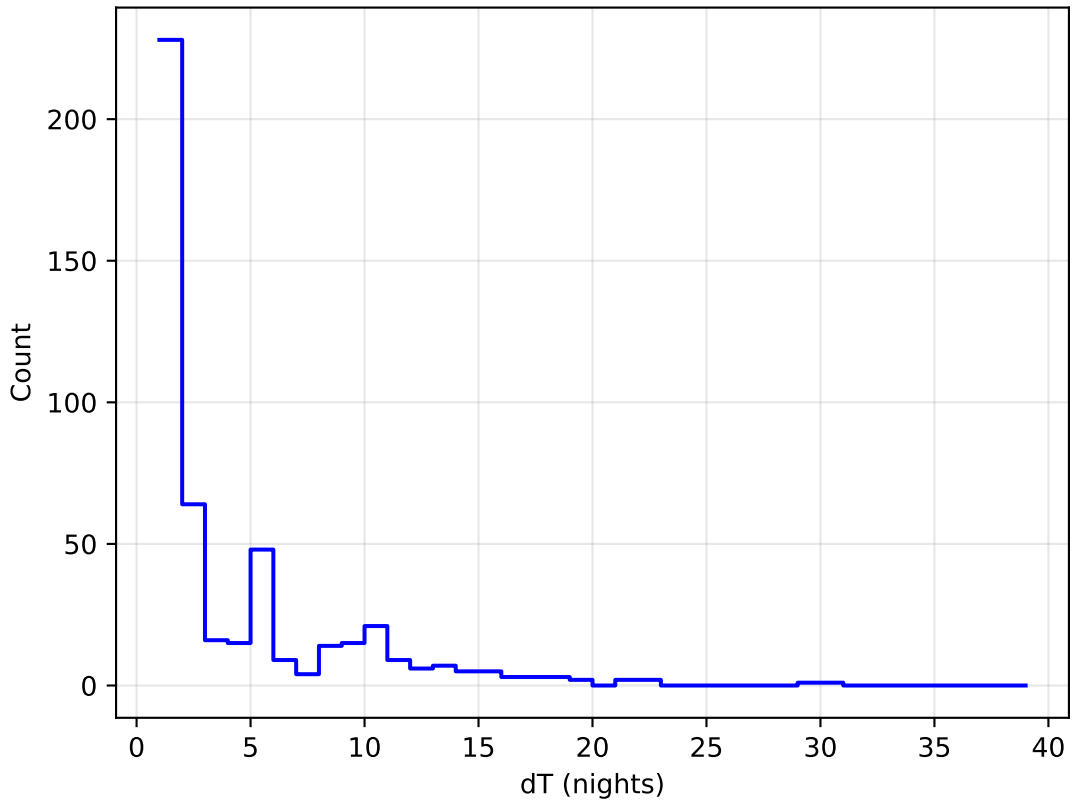
weather_cloudso14v3.4_10yrs all bands: DD: COSMOS Delta Nights Histogram
