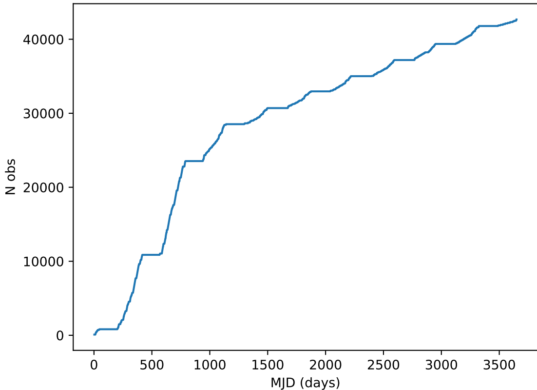
weather_cloudso14v3.4_10yrs all bands: DD:COSMOS Cumulative NVisits
