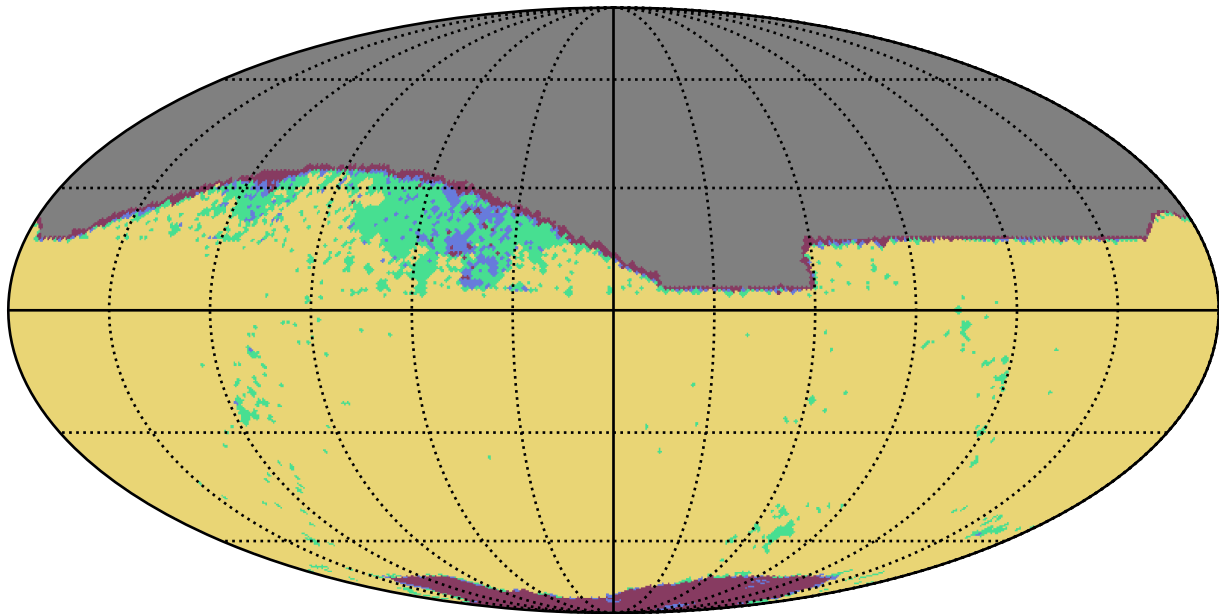
weather_cloudso12v3.5_10yrs z band: YearCoverage night
