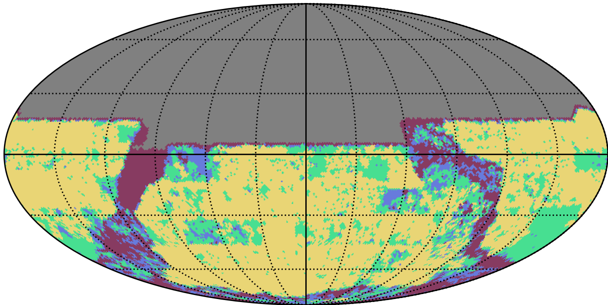
weather_cloudso12v3.5_10yrs u band: YearCoverage night
