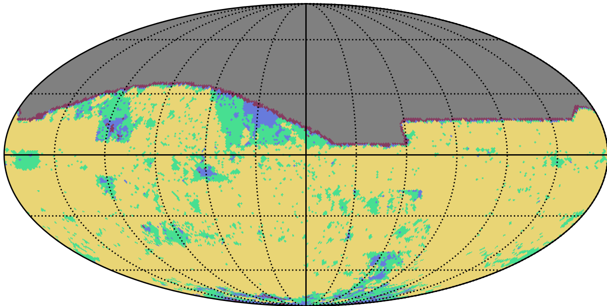
weather_cloudso12v3.5_10yrs g band: YearCoverage night
