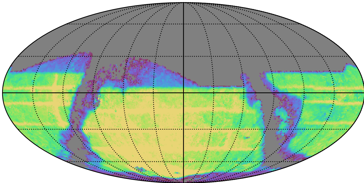
weather_cloudso12v3.5_10yrs : TDC_rate
