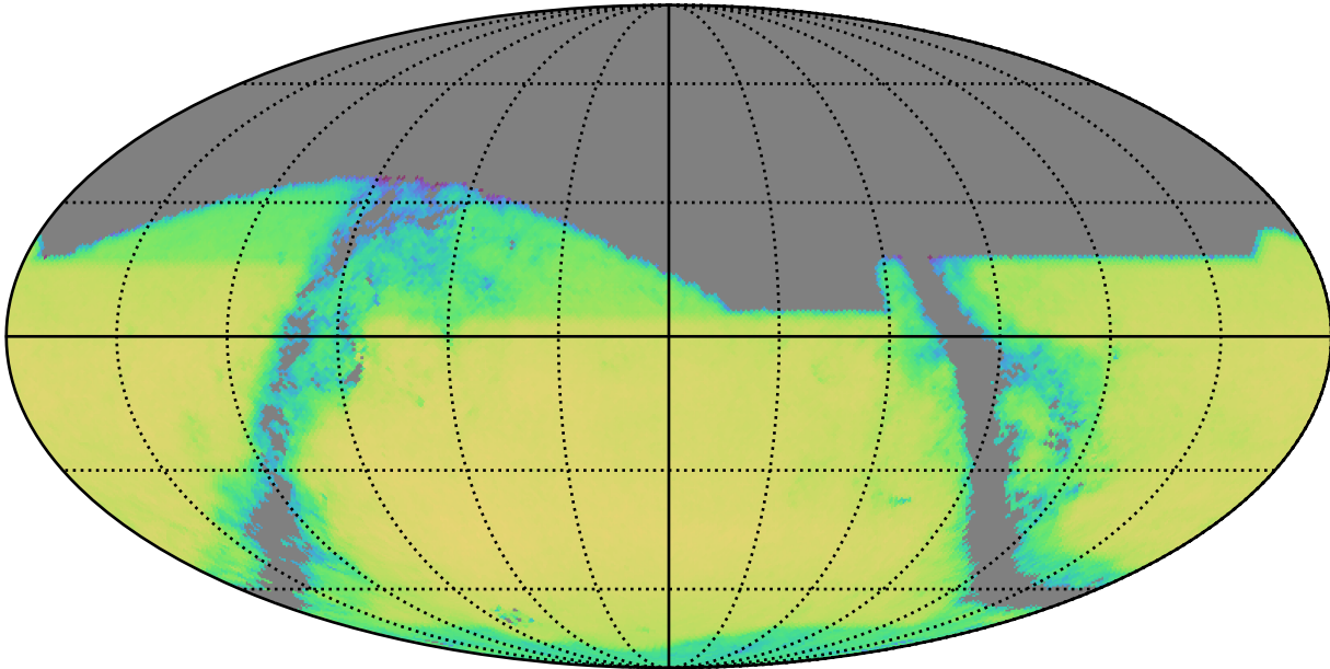
weather_cloudso12v3.5_10yrs r band and non-DD: QSONumberCountsMetric
