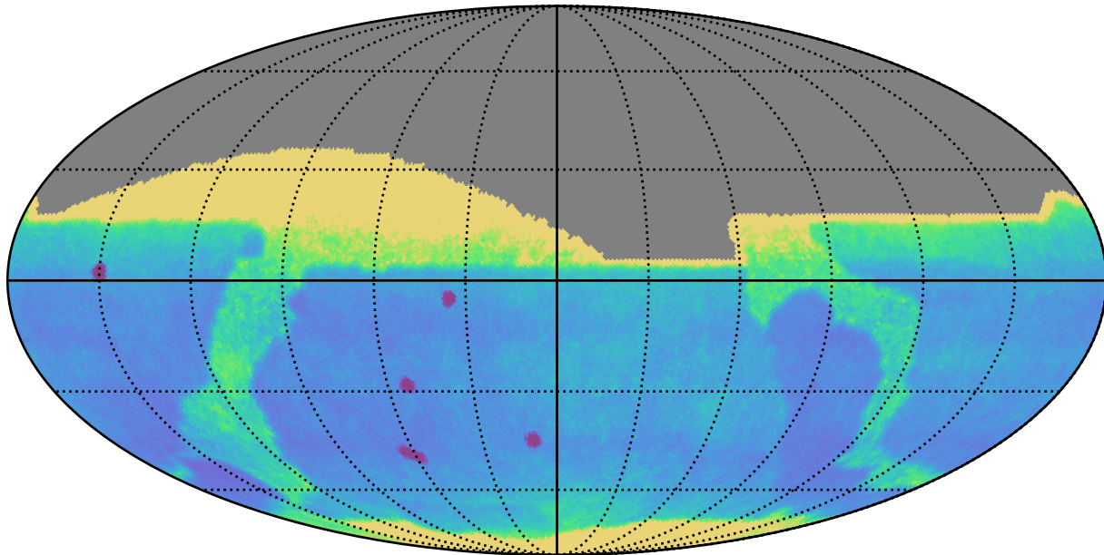
weather_cloudso12v3.5_10yrs : Proper Motion Uncert @ 24.0
