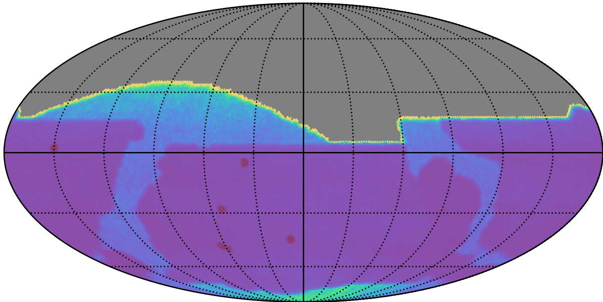
weather_cloudso12v3.5_10yrs : Proper Motion Uncert @ 20.5
