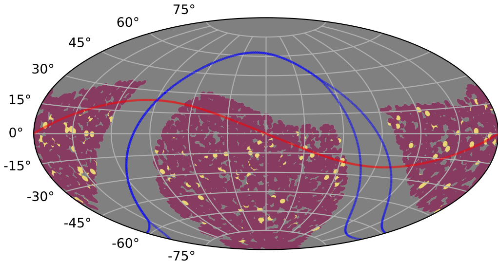
weather_cloudso12v3.5_10yrs : PrestoKNe_score_s
