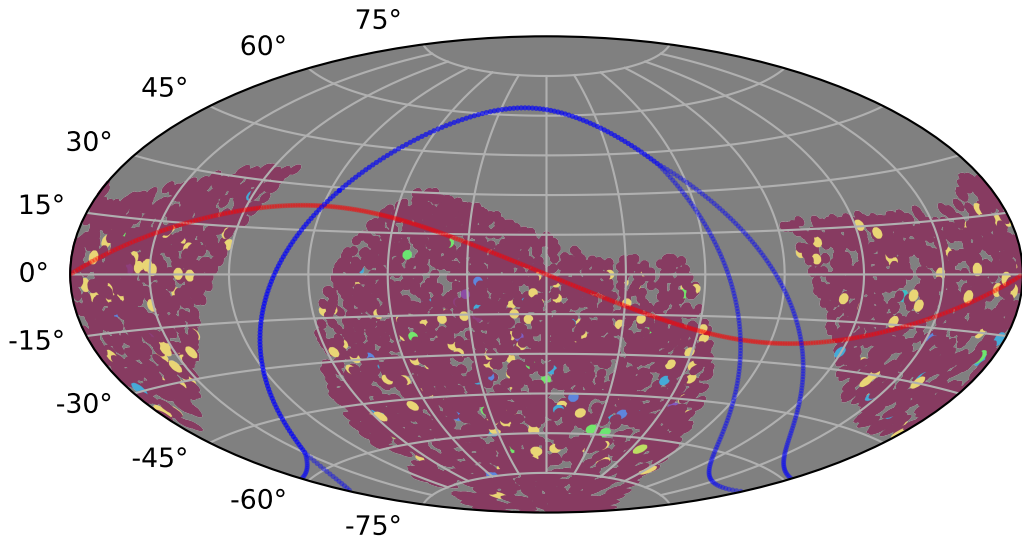
weather_cloudso12v3.5_10yrs : PrestoKNe_score_p
