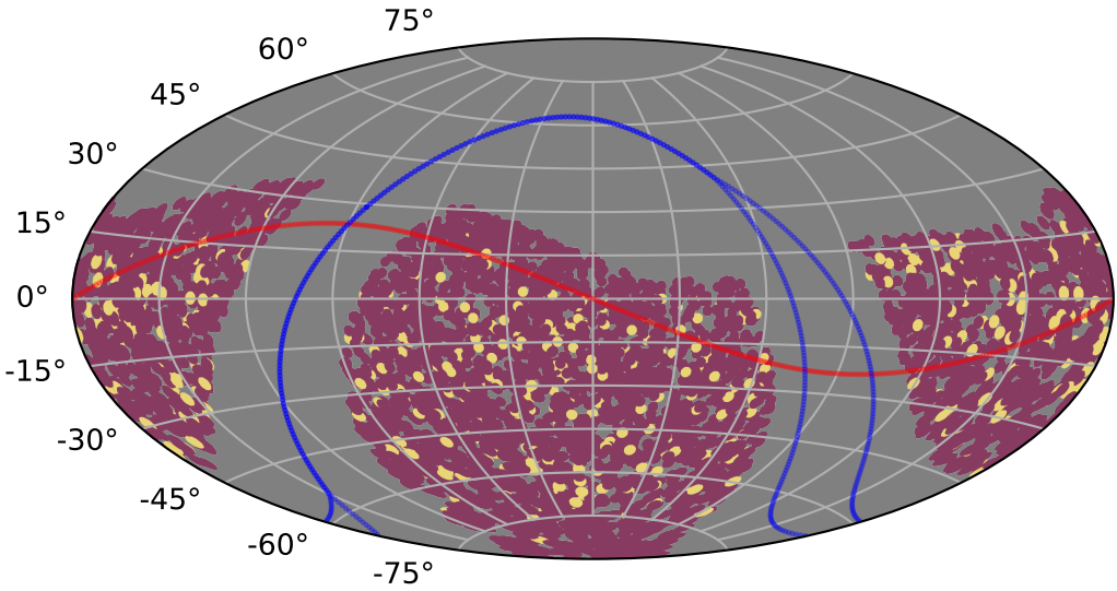
weather_cloudso12v3.5_10yrs : PrestoKNe_presto_color_detect
