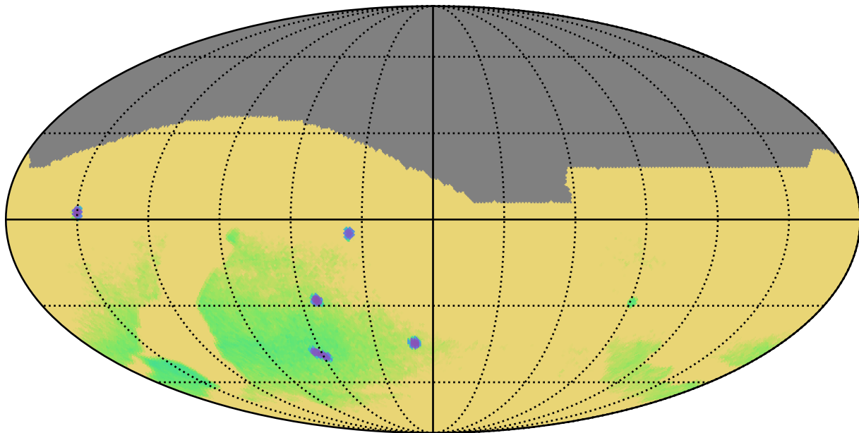
weather_cloudso12v3.5_10yrs : Parallax Uncert @ 22.4
