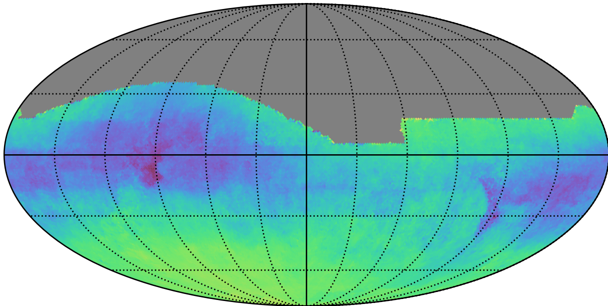
weather_cloudso12v3.5_10yrs : Parallax-DCR degeneracy @ 24.0
