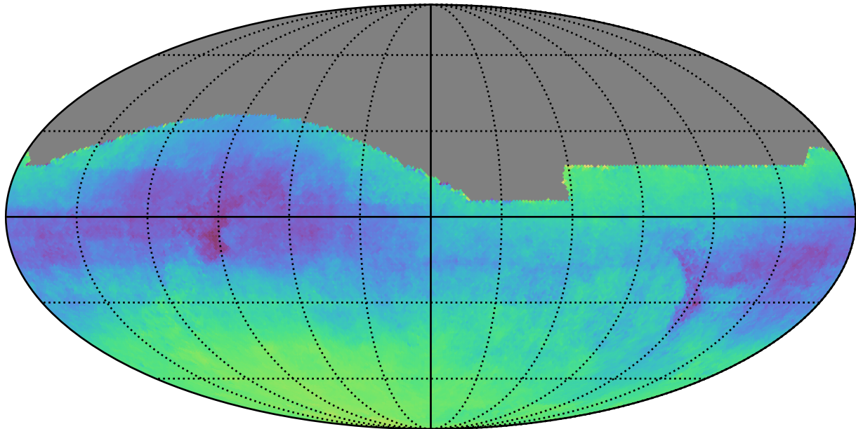
weather_cloudso12v3.5_10yrs : Parallax-DCR degeneracy @ 22.4
