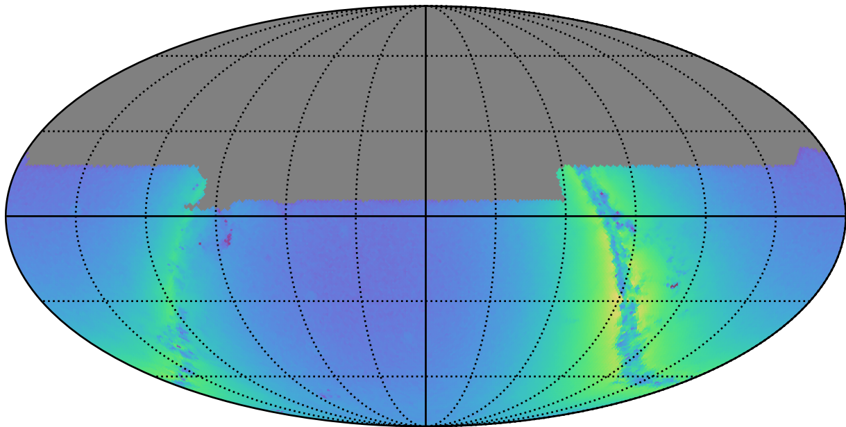
weather_cloudso12v3.5_10yrs u: Nstars_no_crowding
