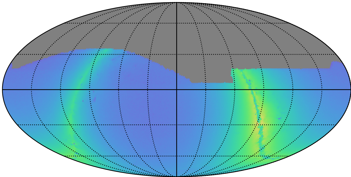
weather_cloudso12v3.5_10yrs i: Nstars_no_crowding
