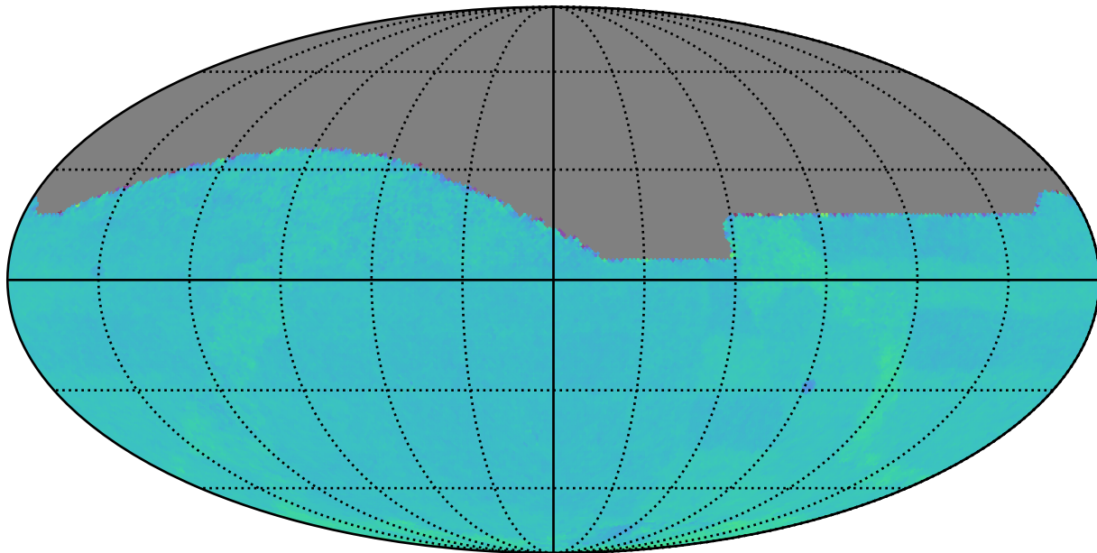
weather_cloudso12v3.5_10yrs : Normalized Proper Motion Uncert @ 20.5
