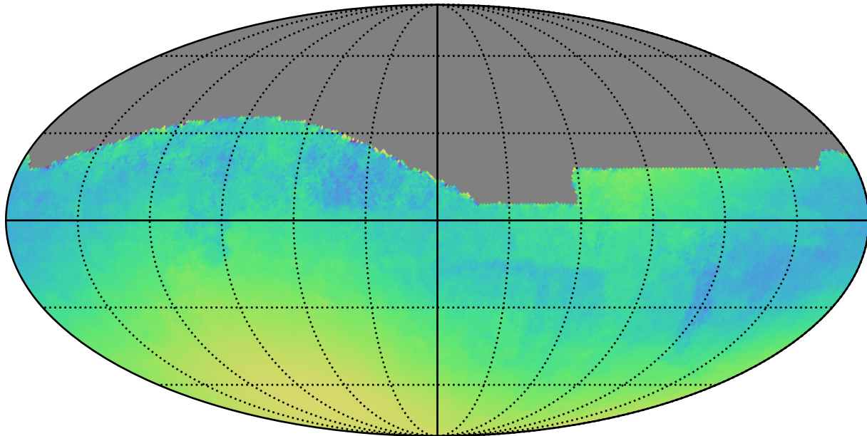
weather_cloudso12v3.5_10yrs : Normalized Parallax Uncert @ 24.0
