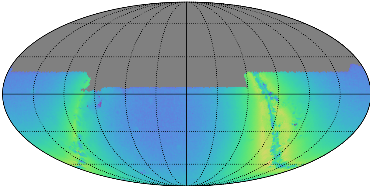
weather_cloudso12v3.5_10yrs u: N stars to Precision 0.20
