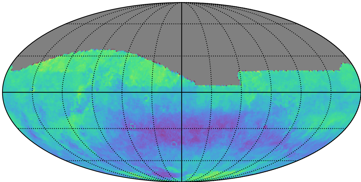
weather_cloudso12v3.5_10yrs z: Kuiper rotSkyPos
