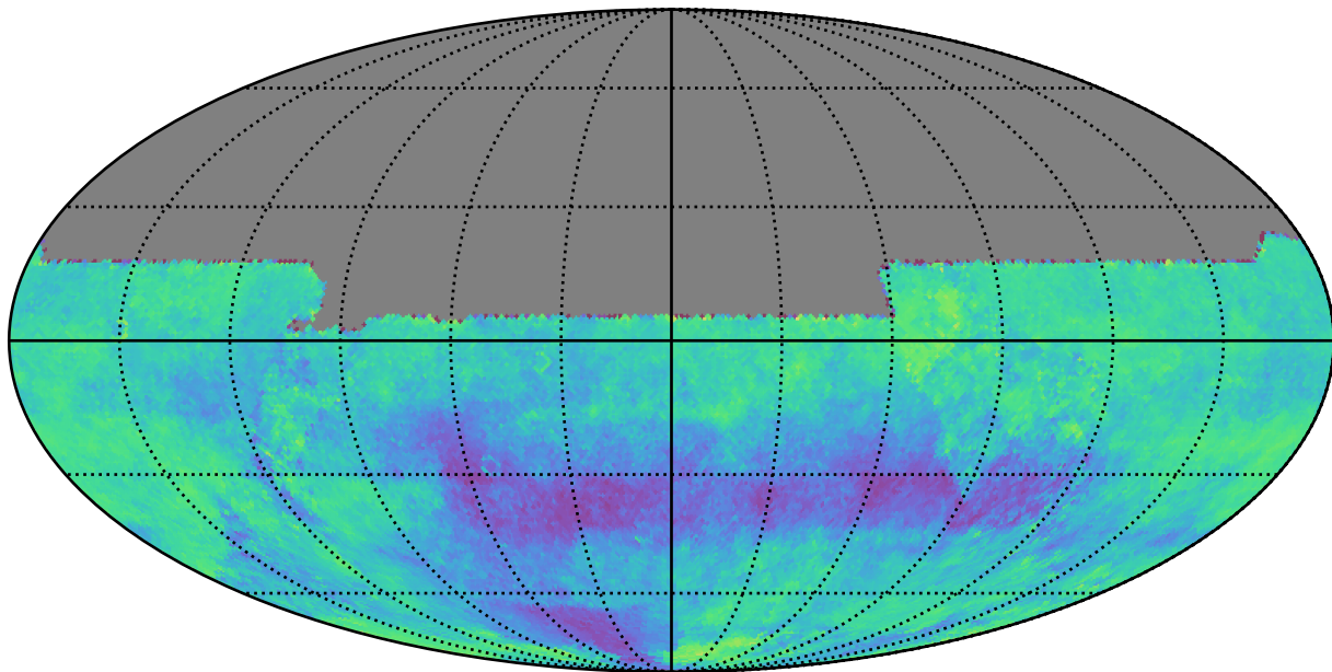
weather_cloudso12v3.5_10yrs u: Kuiper rotSkyPos
