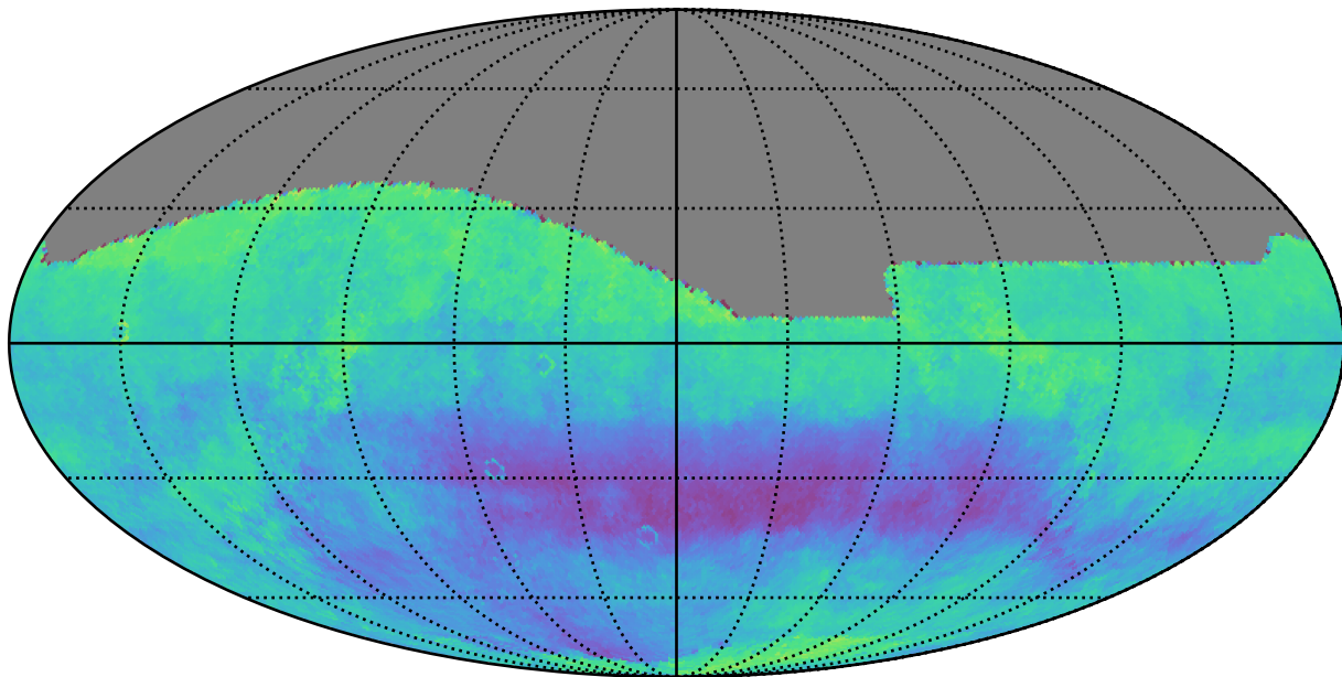
weather_cloudso12v3.5_10yrs r: Kuiper rotSkyPos
