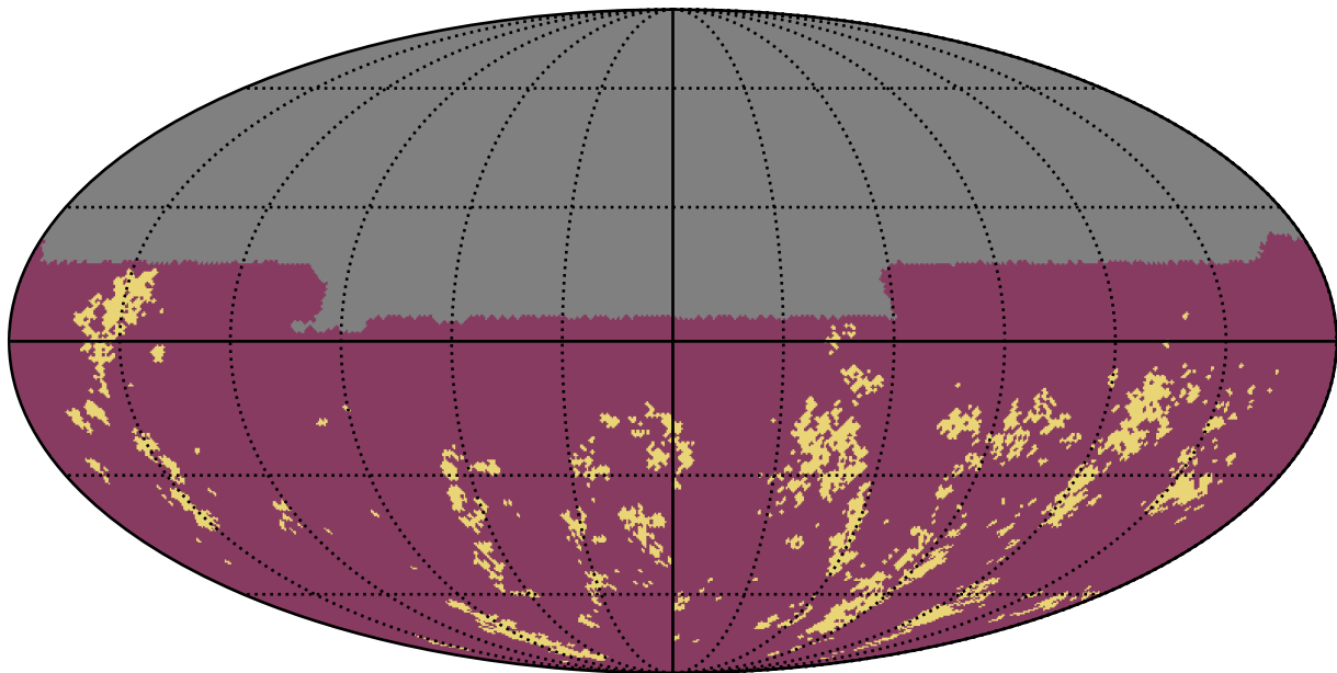
weather_cloudso12v3.5_10yrs u band: Gaps_7hr
