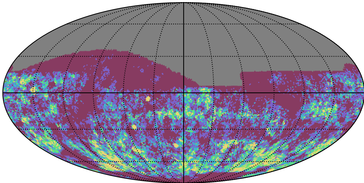
weather_cloudso12v3.5_10yrs i band: Gaps_3hr
