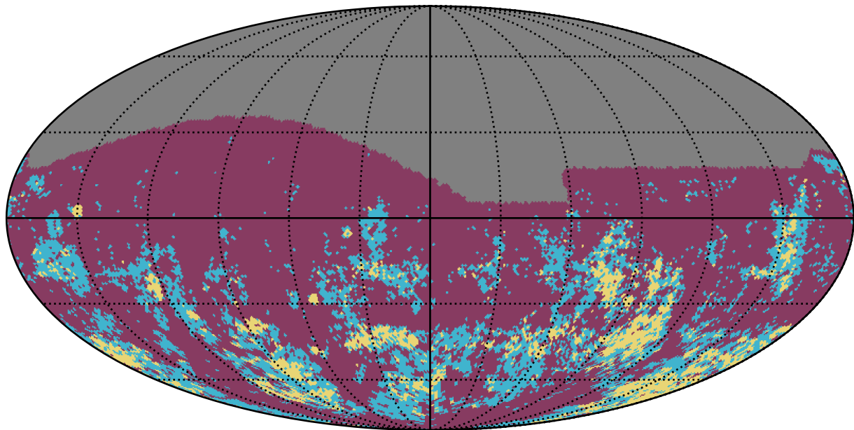
weather_cloudso12v3.5_10yrs g band: Gaps_3hr
