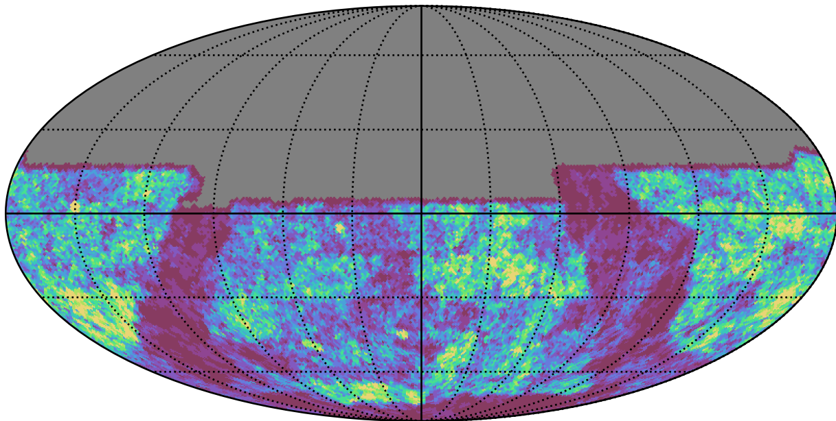
weather_cloudso12v3.5_10yrs u band: Gaps_24hr
