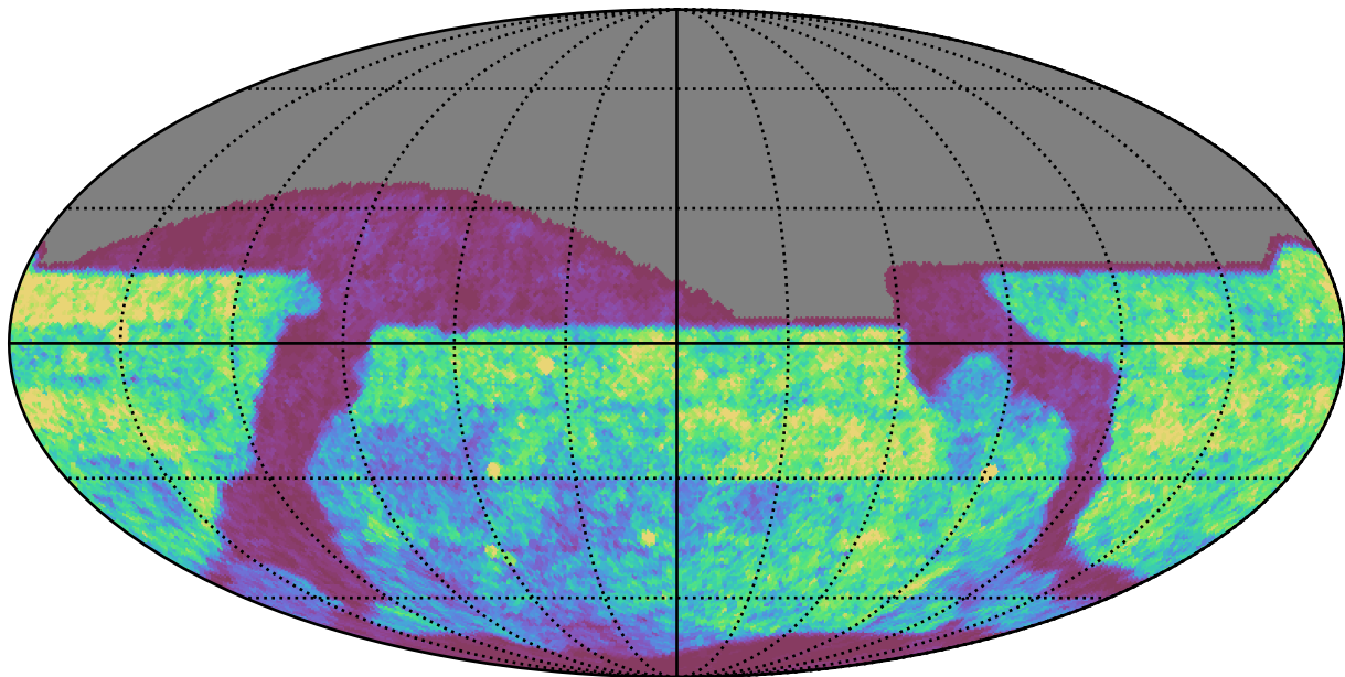
weather_cloudso12v3.5_10yrs r band: Gaps_24hr
