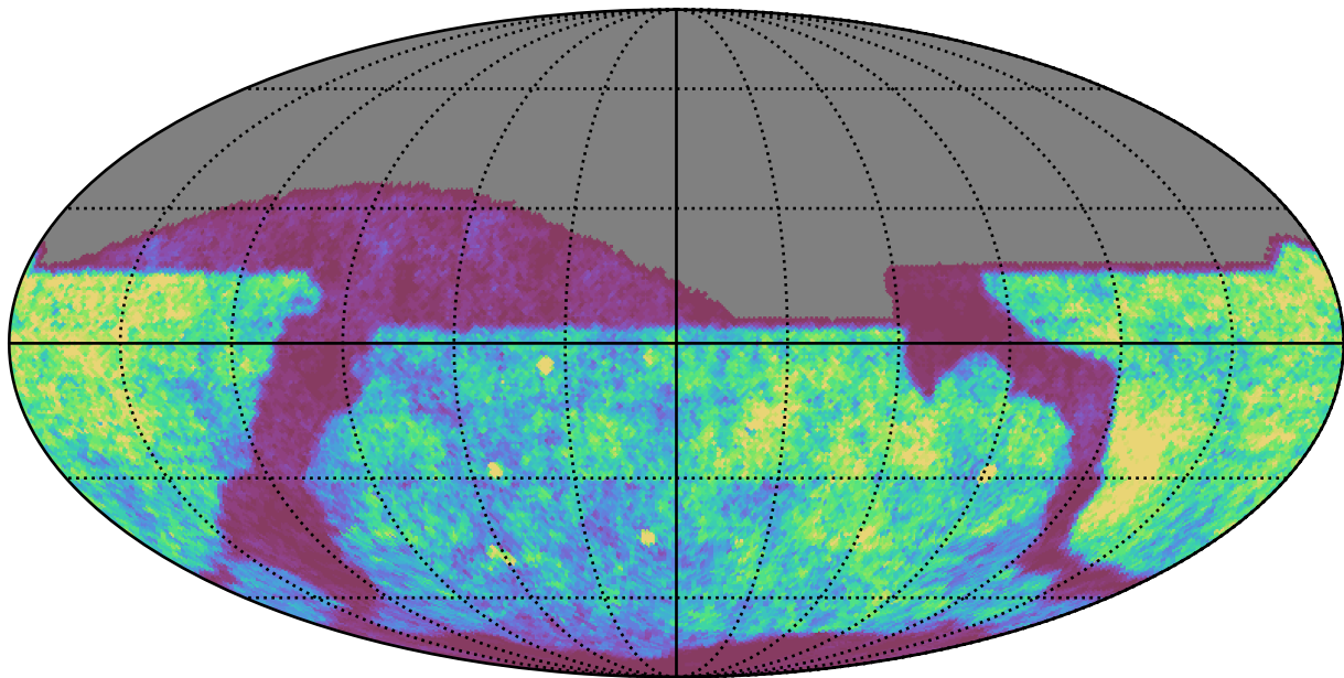
weather_cloudso12v3.5_10yrs i band: Gaps_24hr
