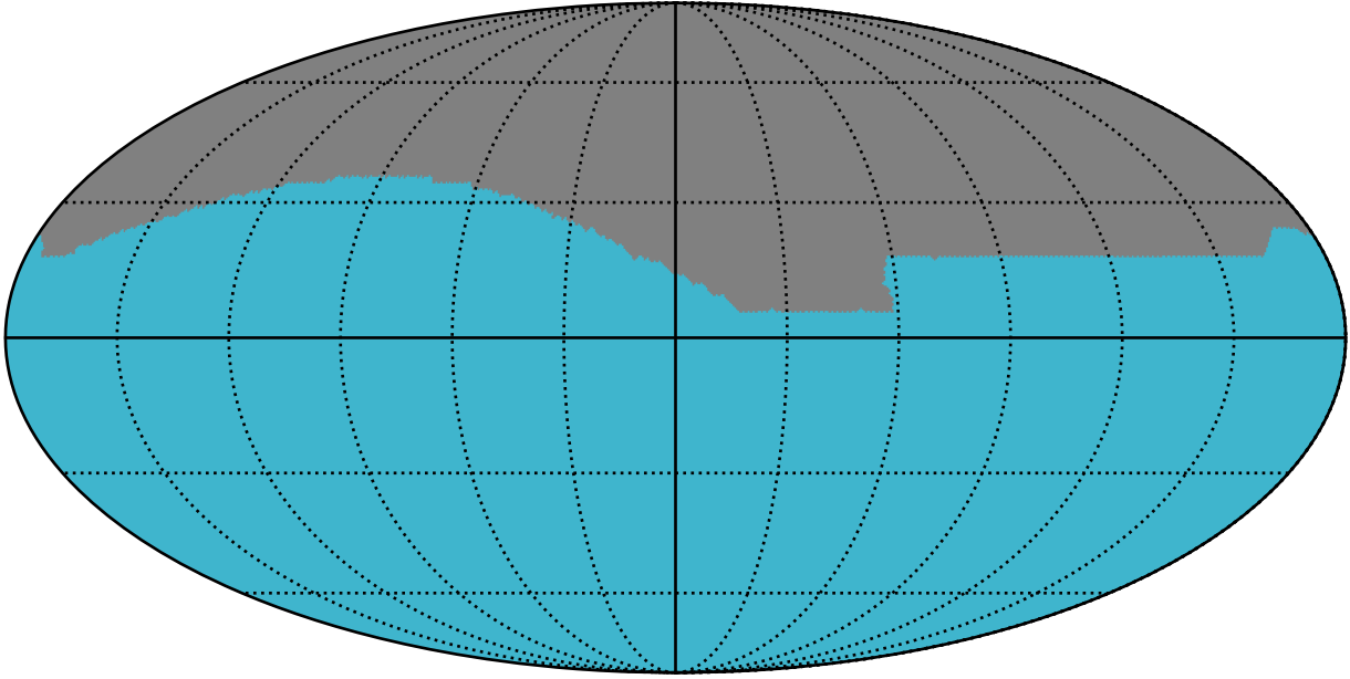
weather_cloudso12v3.5_10yrs : GalplaneFootprintMetric_xray_binaries_map_Tau_2_0
