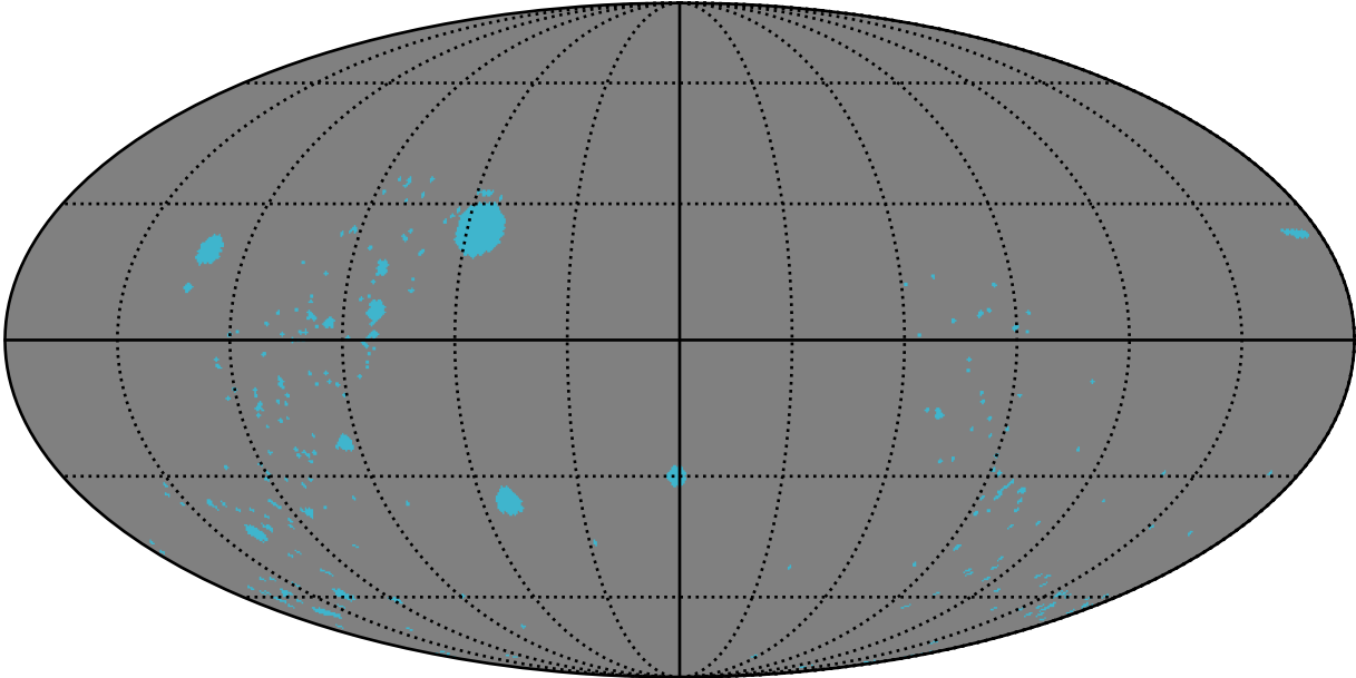
weather_cloudso12v3.5_10yrs : GalplaneFootprintMetric_open_clusters_map_Tau_2_0
