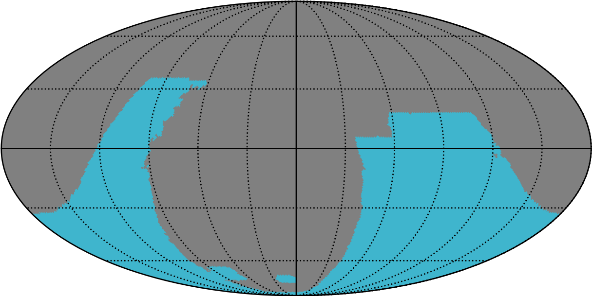
weather_cloudso12v3.5_10yrs : GalplaneFootprintMetric_galactic_plane_map_Tau_2_0
