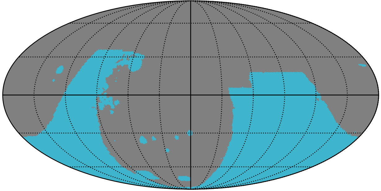
weather_cloudso12v3.5_10yrs : GalplaneFootprintMetric_combined_map_Tau_2_0
