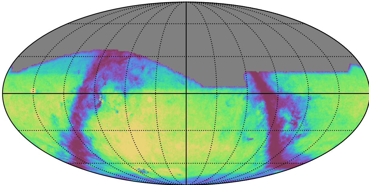
weather_cloudso12v3.5_10yrs g: GalaxyCountsMetricExtended
