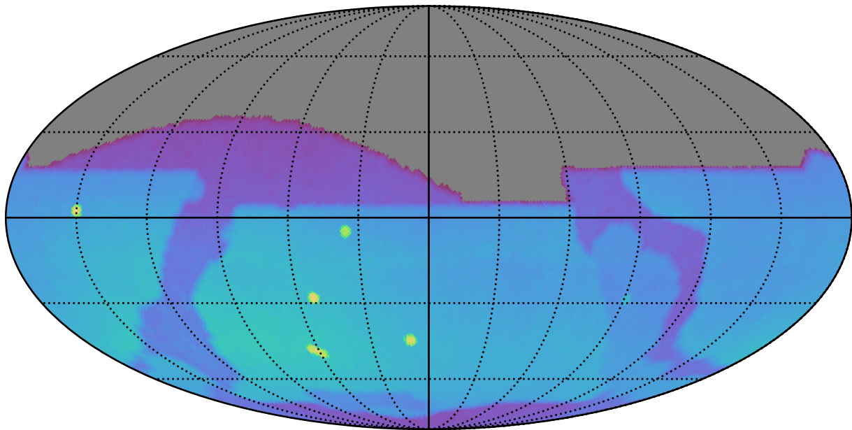
weather_cloudso12v3.5_10yrs : Brown Dwarf, L4
