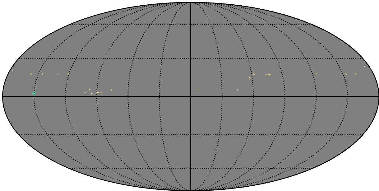
weather_cloudso12v3.5_10yrs y band: AGN_TimeLag_5_days
