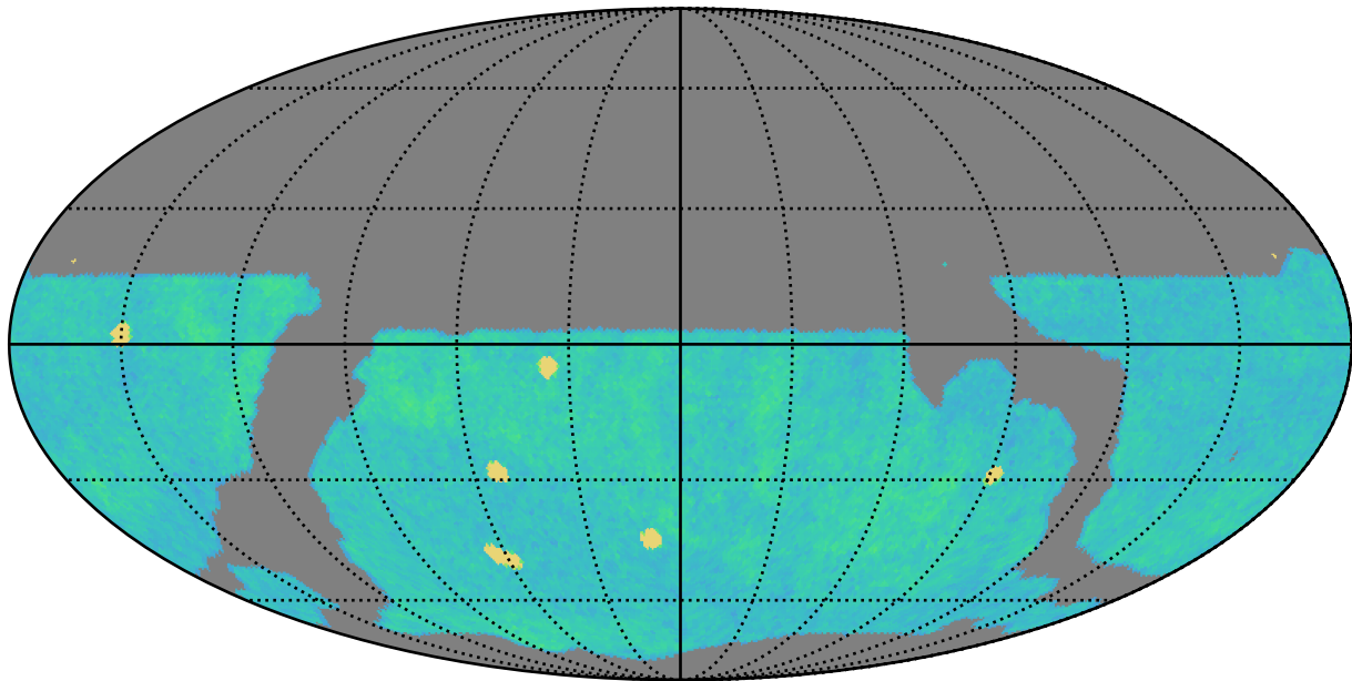
weather_cloudso12v3.5_10yrs i band: AGN_TimeLag_100_days
