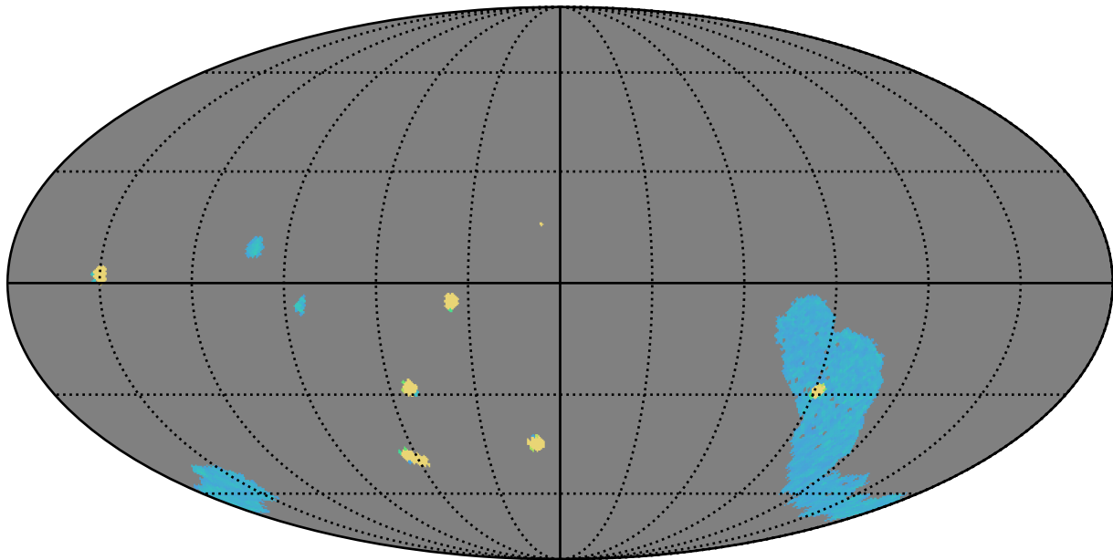
weather_cloudso12v3.5_10yrs g band: AGN_TimeLag_100_days
