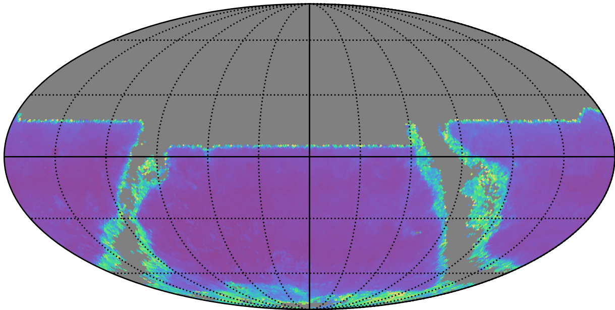
weather_cloudso12v3.5_10yrs y band: AGN SF_uncert
