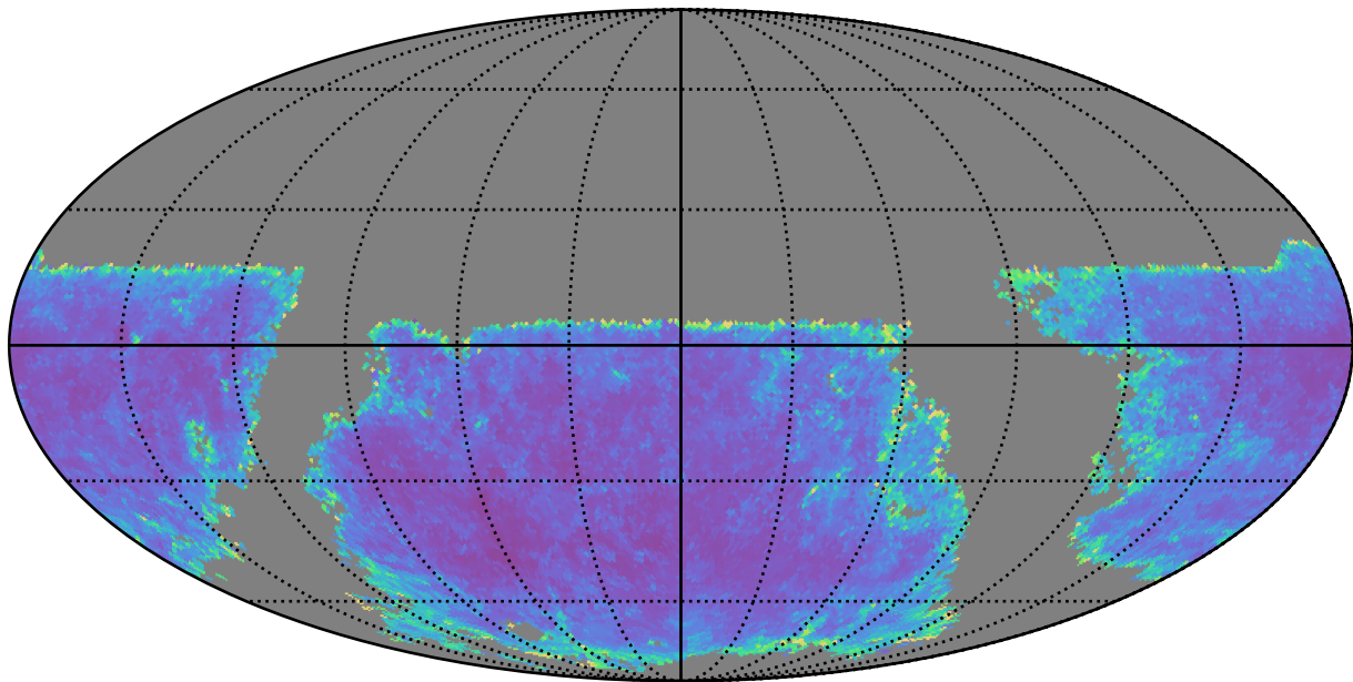
weather_cloudso12v3.5_10yrs u band: AGN SF_uncert
