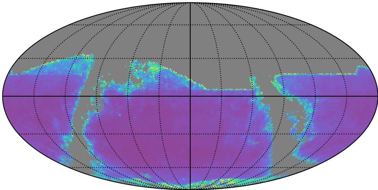
weather_cloudso12v3.5_10yrs r band: AGN SF_uncert
