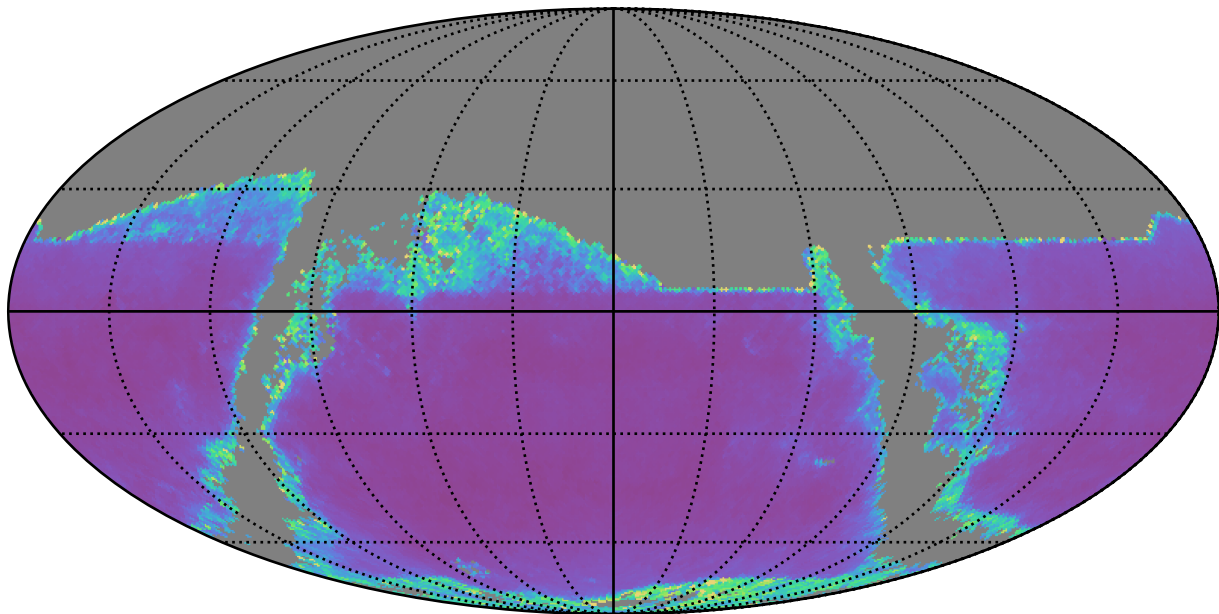
weather_cloudso12v3.5_10yrs i band: AGN SF_uncert
