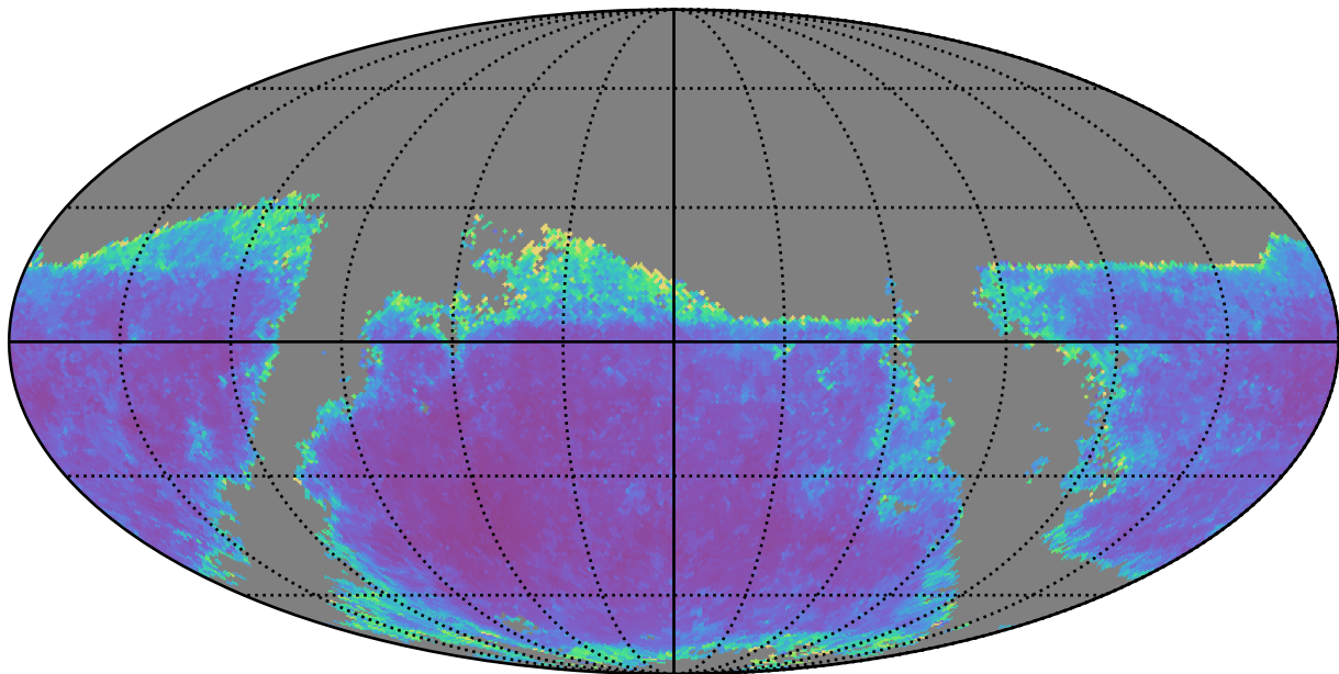
weather_cloudso12v3.5_10yrs g band: AGN SF_uncert
