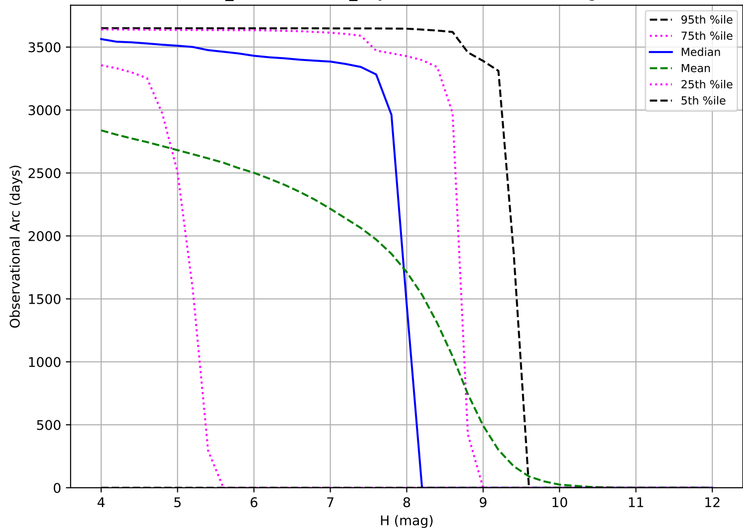
weather_cloudso12v3.4_10yrs: Observational Arc Length TNO
