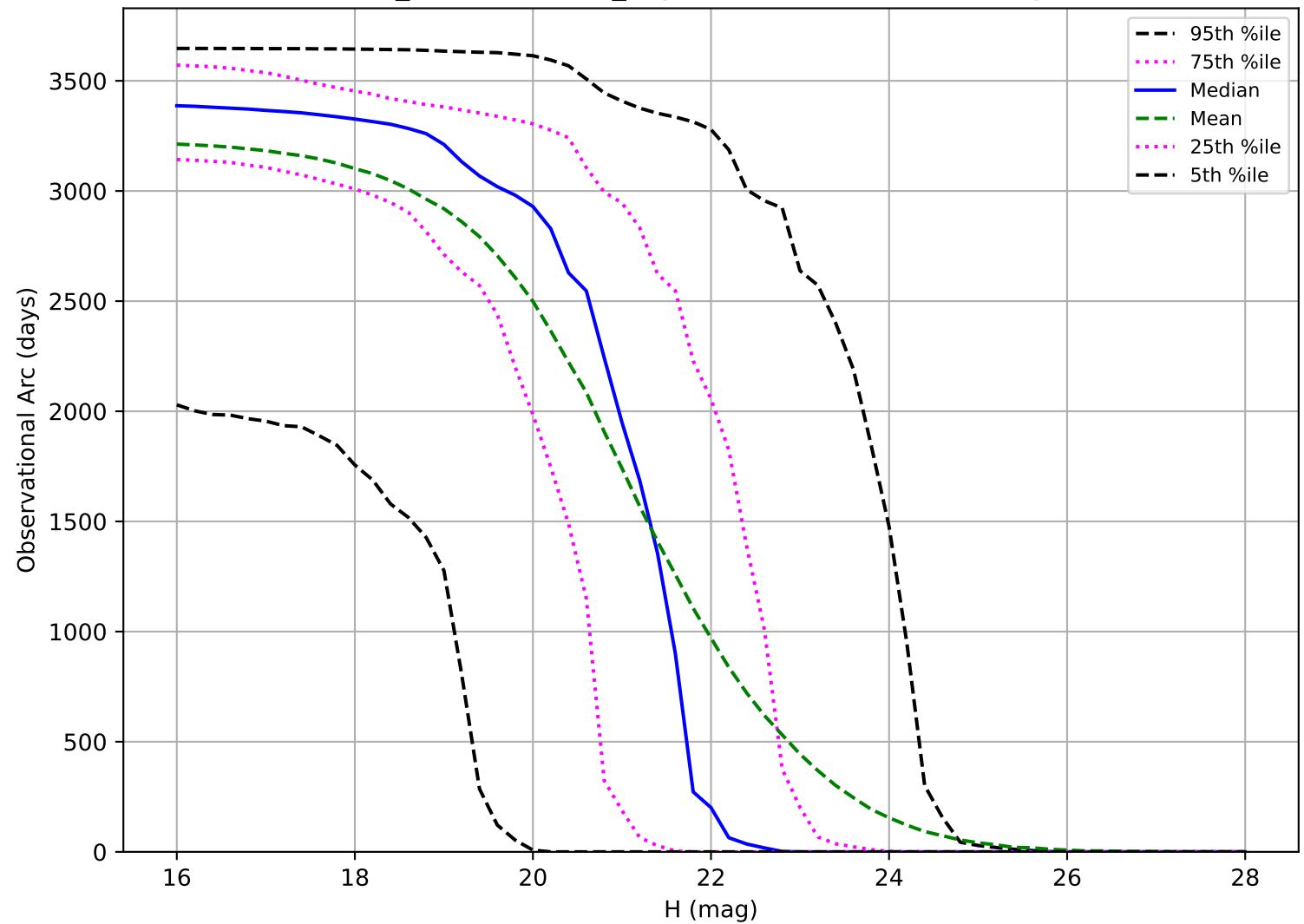
weather_cloudso12v3.4_10yrs: Observational Arc Length PHA
