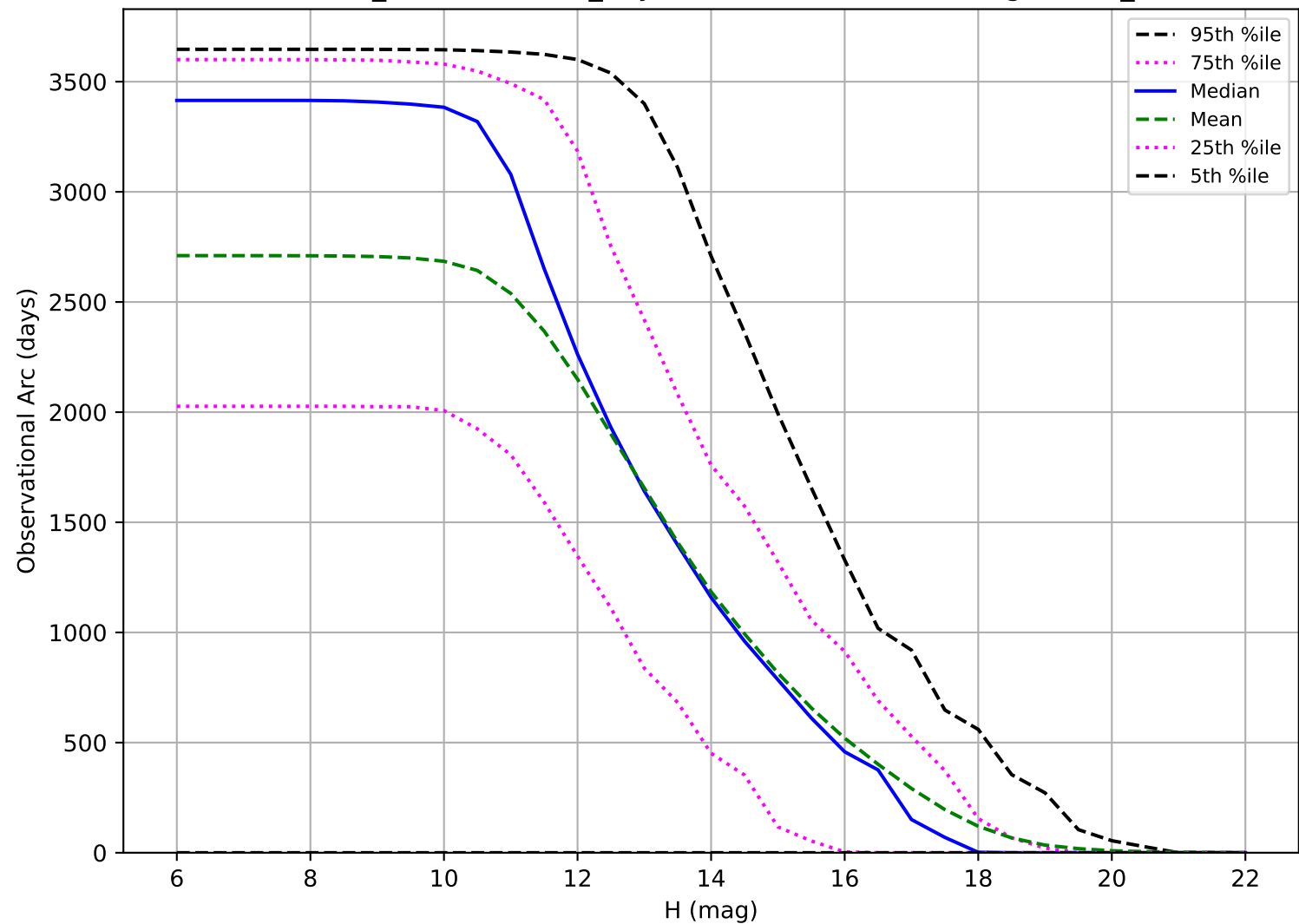
weather_cloudso12v3.4_10yrs: Observational Arc Length OCC_r5
