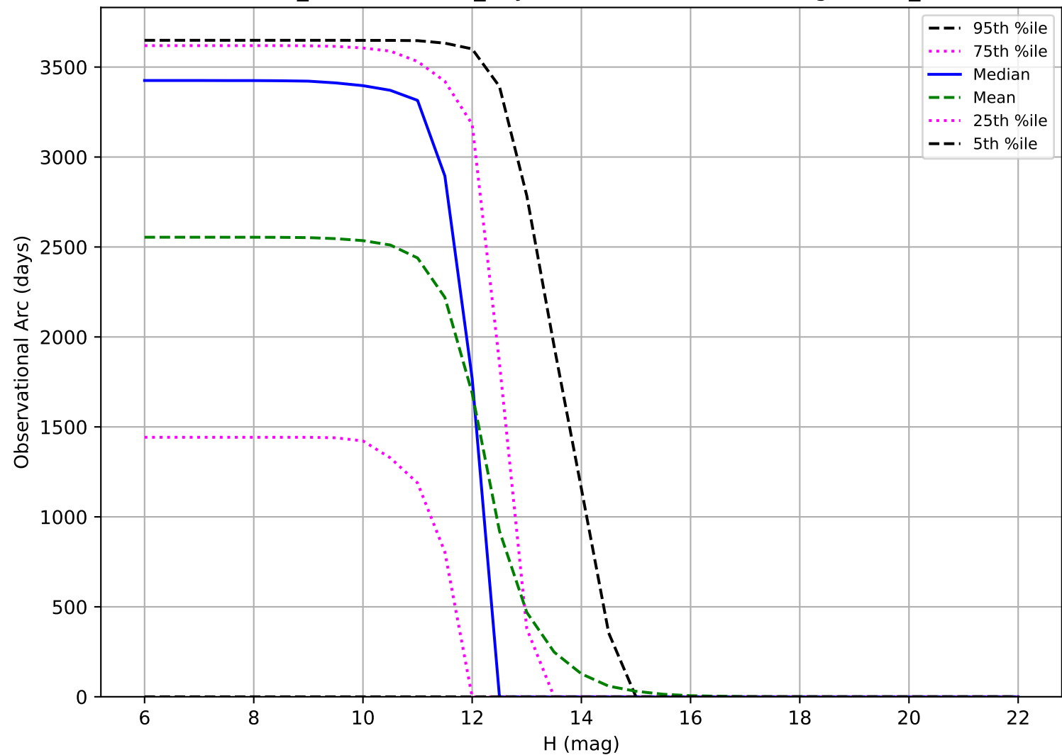
weather_cloudso12v3.4_10yrs: Observational Arc Length OCC_r20
