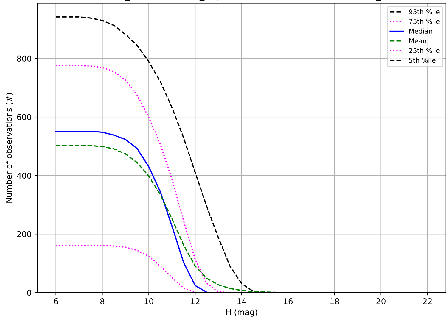
weather_cloudso12v3.4_10yrs: Number of observations OCC_r20
