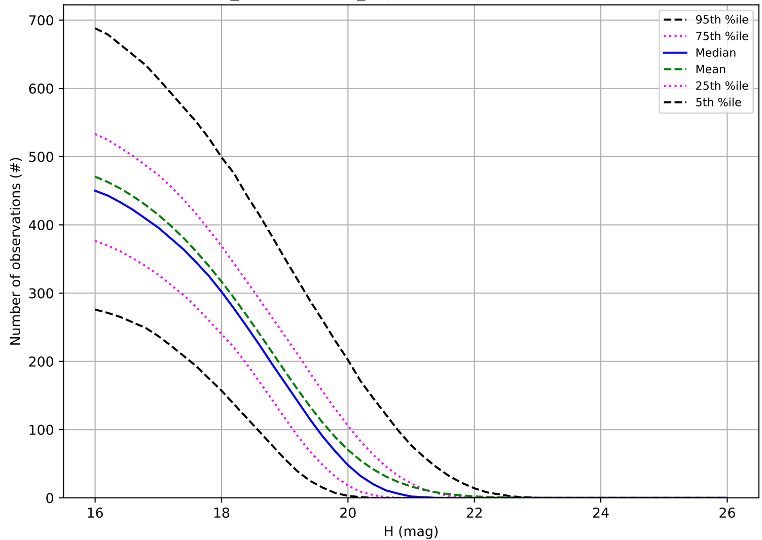
weather_cloudso12v3.4_10yrs: Number of observations MBA
